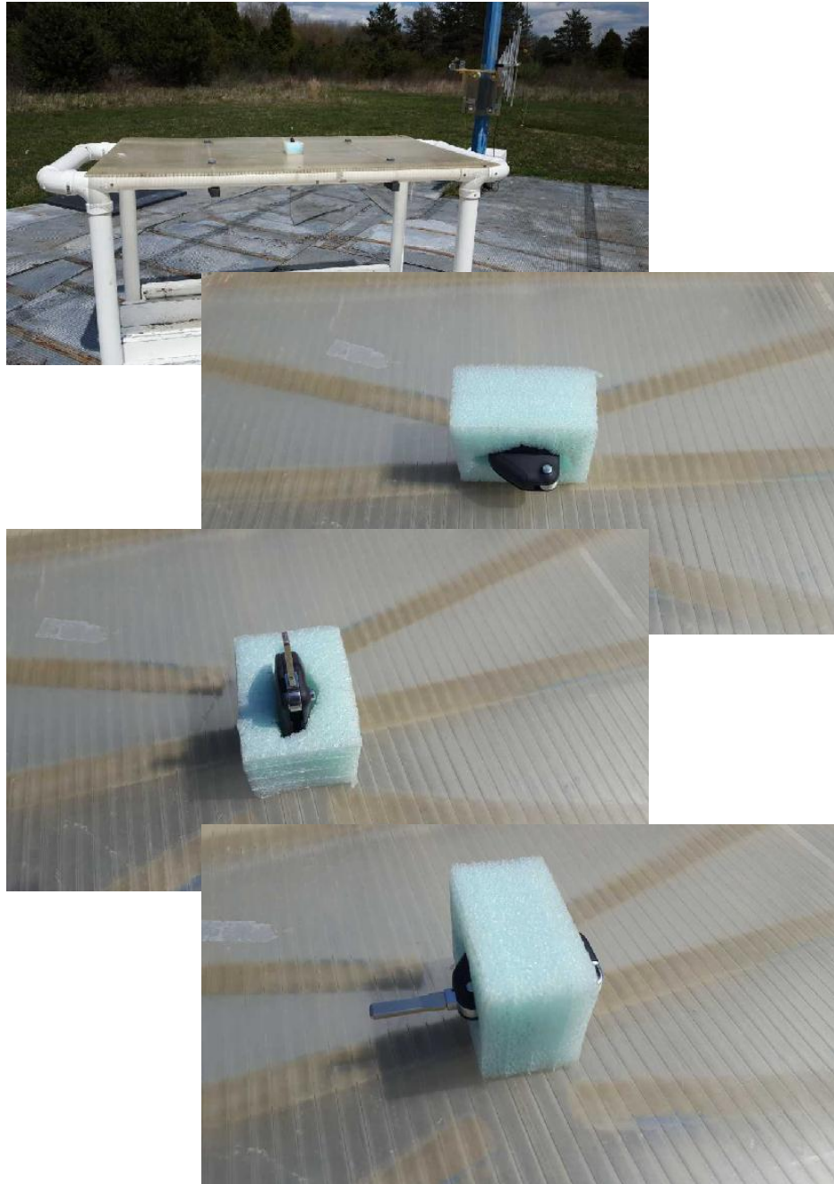
Figure 4: Radiated Emissions Test Setup Photograph(s).
